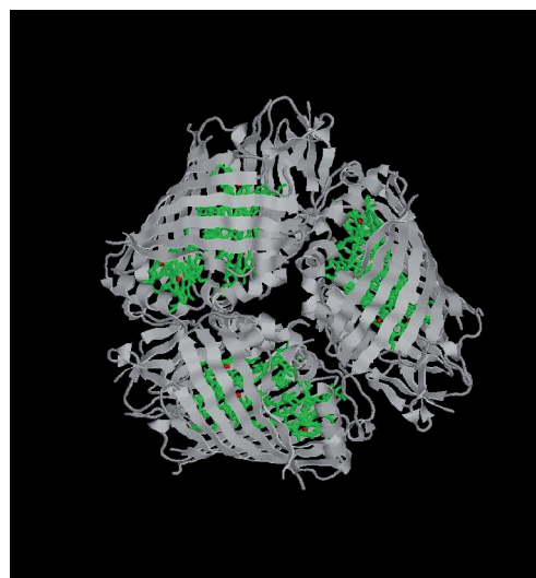
Figure 5: The FMO complex in green sulphur bacteria carries light energy from chlorophyll (green) to reaction centres for chemical processes (red). The energy transport uses an interaction of coherence and decoherence. Wikipedia/Julian Adolphs (license: CC BY-SA 3.0)
