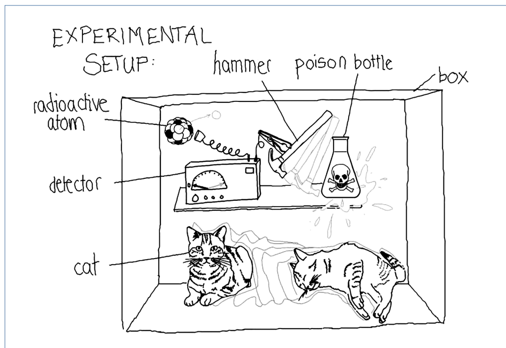
Figure 4: Schrödinger’s cat: Prior to measurement, the cat is in a superposition of the states (1) live cat, non-decayed atomic nucleus and (2) dead cat, decayed atomic nucleus. [Diagram – Lara Hartjes, Ulm]
