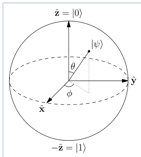
Figure 3: On the three-dimensional Bloch sphere (with x -, y -, and z -axes) the north and south poles correspond to the two classical states, whereas a quantum state can be at any point on the surface of the sphere. The degree of superposition for a state |\psi\rangle from the classical states |0\rangle and |1\rangle on the z -axis is indicated by the polar angle \theta , while the azimuthal angle \phi describes the purely quantum mechanical phase. [Image source: Wikipedia/ User: Smite-Meister (license: CC BY-SA 3.0)]
