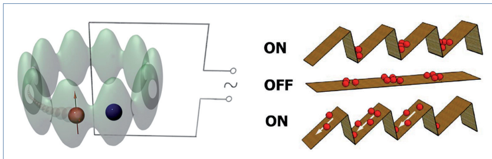
Figure 6: Left: An electric quantum engine – two atoms which can interact locally with one another are placed in a ring-shaped trap of light, with one (red) driven by a time-dependent magnetic field and working against external fields. On the right: A quantum ratchet – by switching an asymmetrical sawtooth potential on and off, particles can be transported due to Brownian movement.
